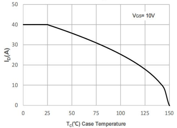
Figure 10: Maximum Continuous Driant Current vs. Case Temperature
